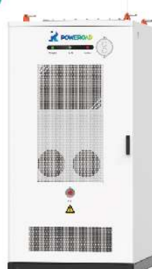
FLEX 261 AIO Liquid Cooling ESS (130kW / 261kWh) (125kW / 261kWh)
